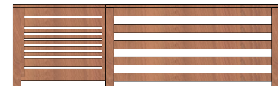
2 3'-0" (900mm) Ht. Cedar Picket Fence Scale: 1:25
